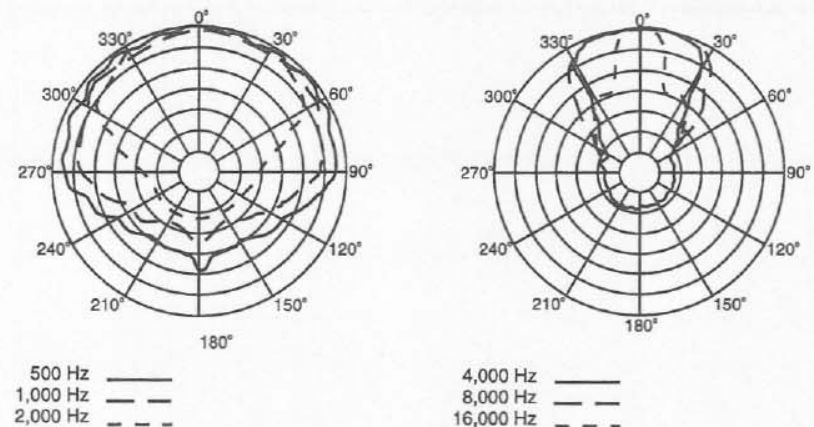
Figure 3—CS810 Polar Response in 1.8 ft³ Sealed Box 4-Volt RMS of 1/3-octave-Band Limited Noise in Anechoic Environment, 20 Feet on Axis (5 dB per Division)
