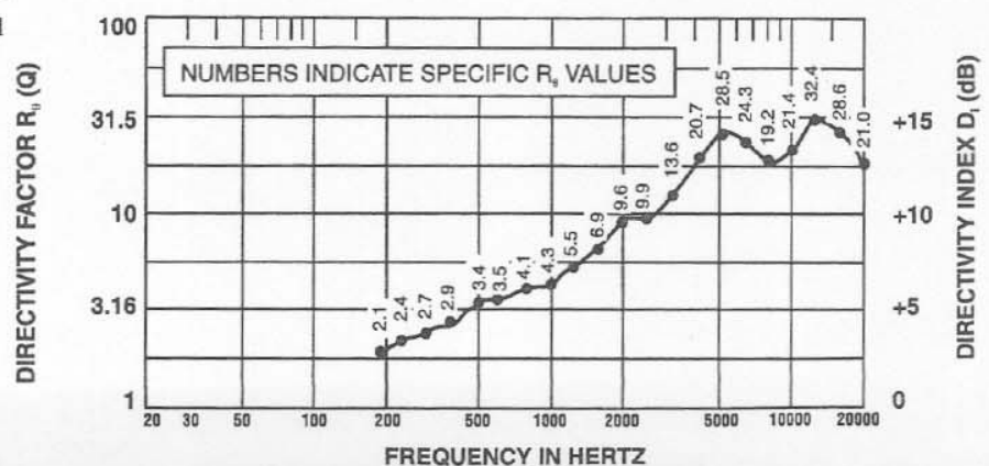
Figure 5—CS810 Directivity Factor and Directivity Index vs. Frequency in a 1.8 ft³ Sealed Box
